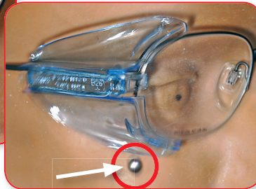
Below: A B-26+ SideShield successfully deflecting a 1/4 inch steel ball at 150 fps (102 mph) during testing.
